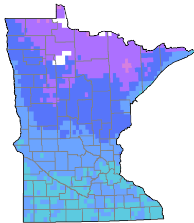
GFDL A1FI
