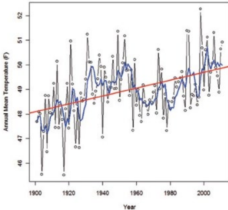
Mean Annual Temperature – increasing 0.016°F per year.
