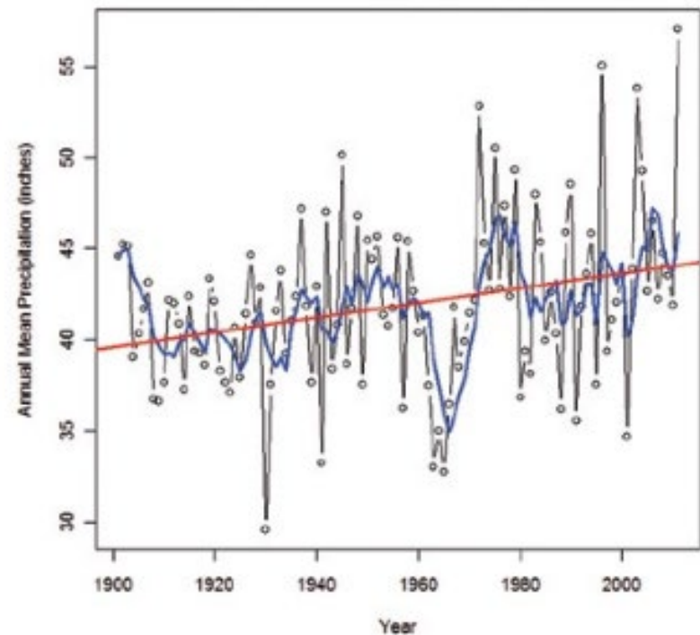
Mean Annual Precipitation – increasing 0.04 inches per year.
