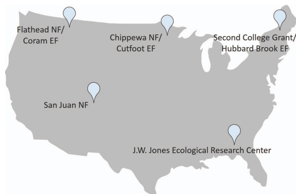
Figure 3. The Cutfoot Experimental Forest (EF) ASCC installation is located in red pine-dominated stands of the Chippewa National Forest (NF) in northern Minnesota. The San Juan NF in mountainous southwest Colorado hosts the ASCC site in mixed conifer forests whose dominant species change with elevation. The Jones Center installation at Ichauway, southern Georgia, focuses on mixed pine systems of the southeastern coastal plain. ASCC sites are being planned for western larch-dominated forests on the Flathead National Forest and the Coram Experimental Forest in northern Montana, and for a northern hardwoods forest at Dartmouth's Second College Grant, with a companion installation planned for Hubbard Brook Experimental Forest in New Hampshire.
